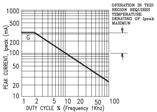
Fig5. Maximum Peak Current vs. Duty Cycle %
