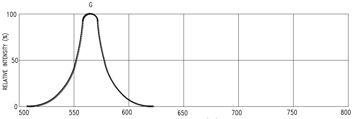
Fig1. Spectral Emission
