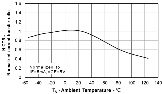
Fig.7 Relative Current Transfer Ratio vs. Ambient Temperature
