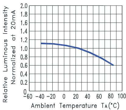
Fig.5 Relative Luminous Intensity vs. Ambient Temperature
