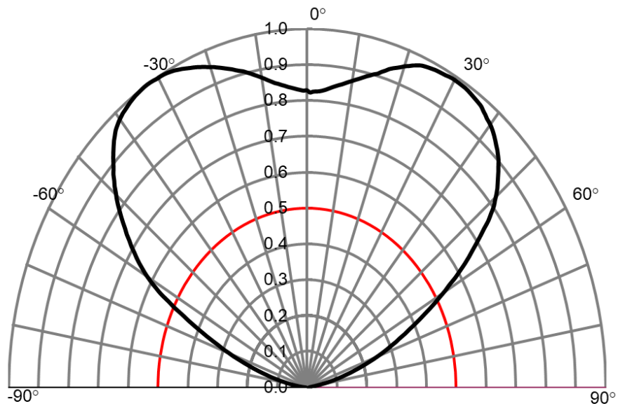
Fig 2. Radiation Characteristics
