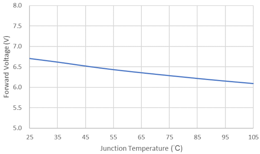
Fig.4 Forward Voltage vs Junction Temperature
