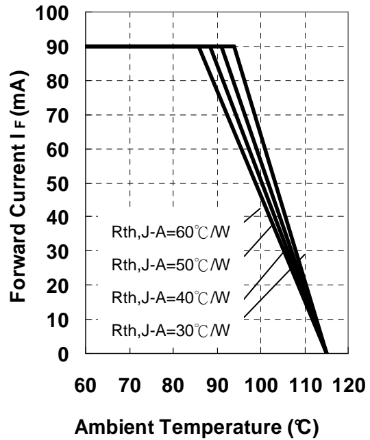
Fig 4. Forward Current Derating Curve
