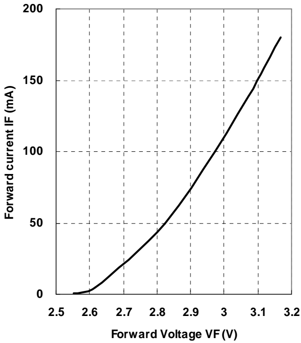
Fig 3. Forward Current
