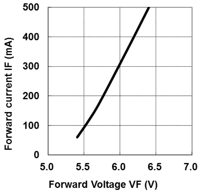
Fig 3. Forward Current
