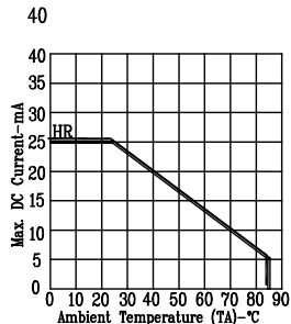
Fig. 5. MAX. ALLOWABLE DC CURRENT VS. AMBIENT TEMPERATURE.
