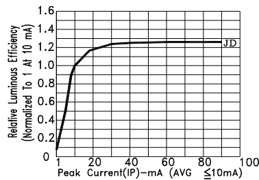
Fig2. RELATIVE LUMINOUS EFFICIENCY (LUMINOUS INTENSITY PER UNIT CURRENT) VS. PEAK CURRENT
