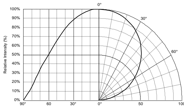
Fig 2. Radiation Characteristics
