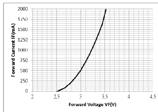
Fig 3. Forward Current
