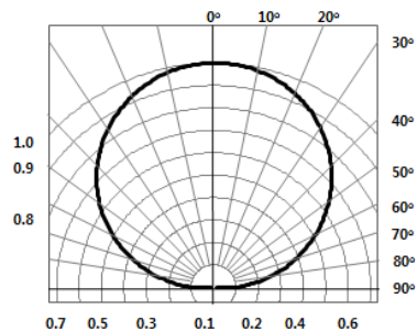
Fig. 5 Spatial Distribution
