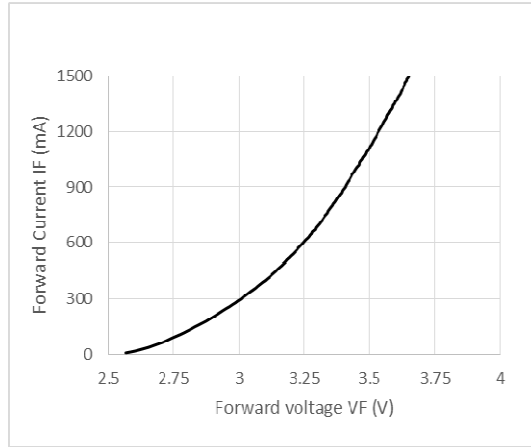
Fig 4. Forward Current
