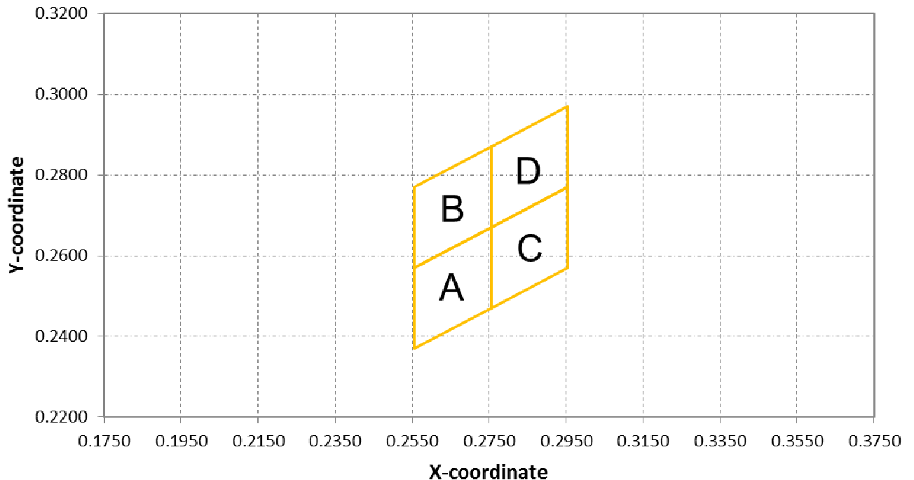
C.I.E 1931 Chromaticity Diagram
