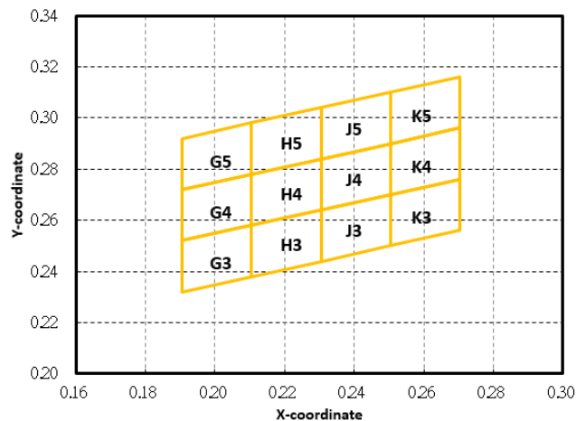
C.I.E. 1931 Chromaticity Diagram
