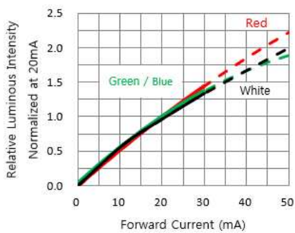
Fig. 4 RELATIVE LUMIOUS INTENSITY VS. FORWARD CURRENT
