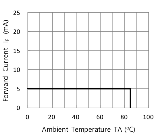
Fig. 2 FORWARD CURRENT VS. DERATING CURVE
