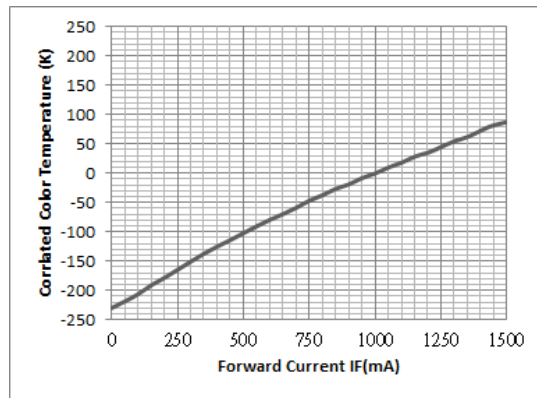
Fig 5. Correlated Color Temperature (CCT) Shift
