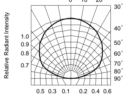
FIG.5 SENSITIVITY DIAGRAM
