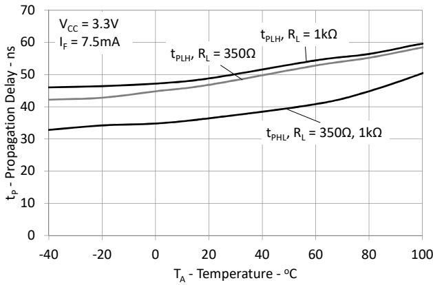
Figure 8: Typical Propagation Delay vs. Ambient Temperature
