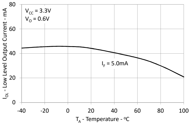
Figure 6: Typical Low Level Output Current vs. Ambient Temperature
