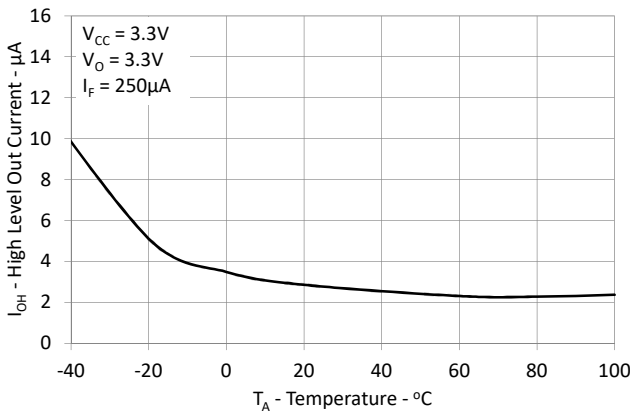
Figure 3: Typical high level output current vs. temperature.
