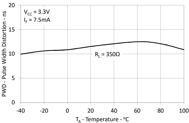
Figure 9: Typical Pulse Width Distortion vs. Ambient Temperature
