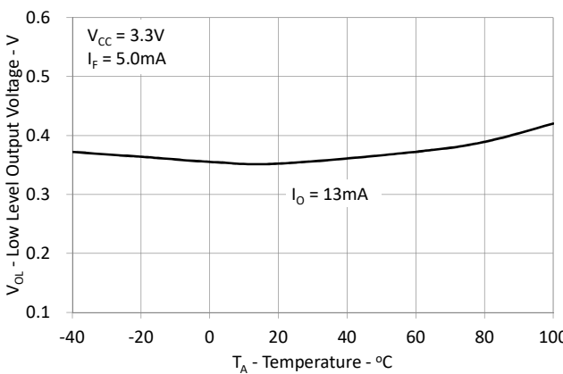
Figure 5: Typical Low Level Output Voltage vs. Ambient Temperature
