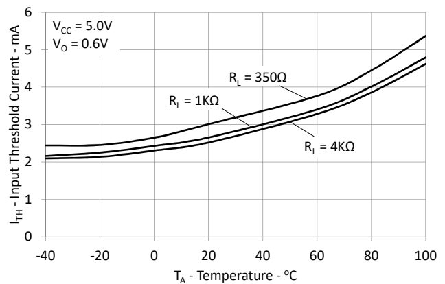
Figure 4: Typical Input Diode Threshold Current vs. Ambient Temperature
