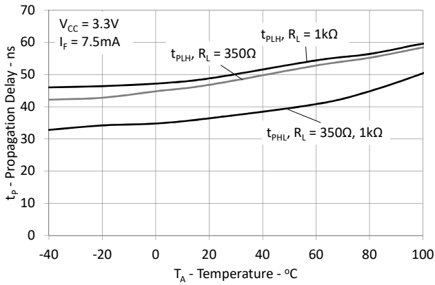
Figure 8: Typical Propagation Delay vs. Ambient Temperature
