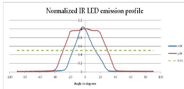
Figure 4.4 LED Angular of incidence
